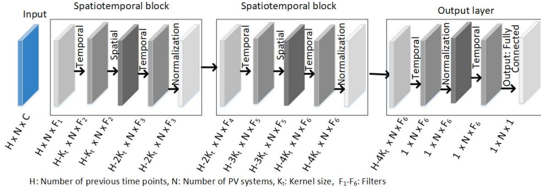
Figure 2: Architecture of spatiotemporal graph neural network . The dimension of input layer is H \times N \times C , where H is the number of previous data points in timeseries. If 2 hours of previous data points are used and the frequency is 5 minutes then the value of H becomes 24. N is number of PV systems or nodes in a graph (316 PV systems) and C is number of channels in the input dataset.
