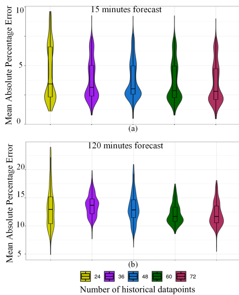
Figure 6: The plots show performance of spatiotemporal forecasting models when the number of previous data points are increased from 24 (2 hours) to 72 (6 hours). (a) shows the plot when forecasting 15 minutes in the future and (b) shows the plot when forecasting 120 minutes in the future.
