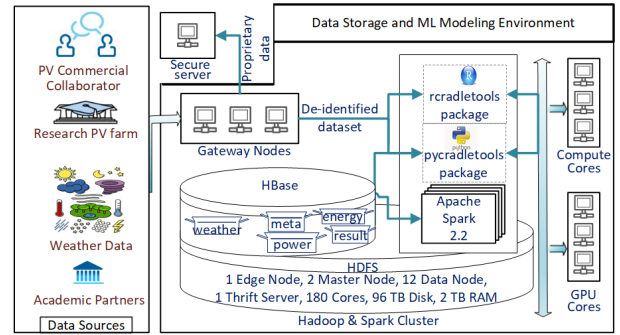
Figure 4: Schematic representation of the data workflow. The figure shows various data sources, and a program periodically executed by a cron job collects the datasets from these sources onto the Hadoop cluster. rcradletools and pycradletools are two packages developed internally to provide the functionality to interact with HBase and perform data processing tasks on the R or python environment, respectively.
