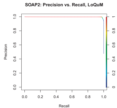
Fig. 5. Precision versus recall for the alignment tool SOAP2, using the raw mapping qualities in (a), and the output of LoQuM in (b). The color of the curve denotes a threshold on mapping quality or prediction output; decreasing this threshold typically increases recall but decreases precision
